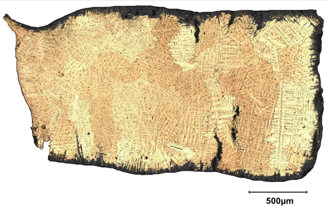
Fig. 6: Micrograph of the etched cross-section of the sample taken from the bracelet (Fig. 2) in bright field,
