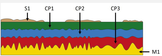
Fig. 3: Stratigraphic representation of the corrosion structure of the bracelet by macroscopic and binocular observation,
