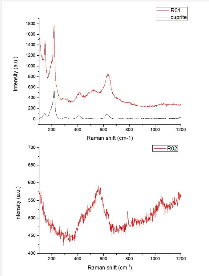
Fig. 11: Raman spectra of points R01 (together with the RRUFF reference RRUFFID=R140763 for cuprite) and R02 showed in Fig. 10,
