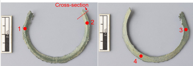
Fig. 2: Side A (left) and side B (right) of bracelet showing the sampling area and the XRF analysis areas (red dots),
