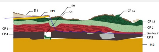
Fig. 6: Preliminary stratigraphy 1, corresponding to the front face of the aegis. S = soil, D = deposit, M = metal, CP = corrosion products, SV = structural void,
