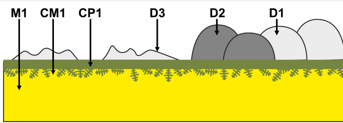
Fig. 4: Stratigraphic representation of the corrosion structure of the bracelet by macroscopic and binocular observation,
