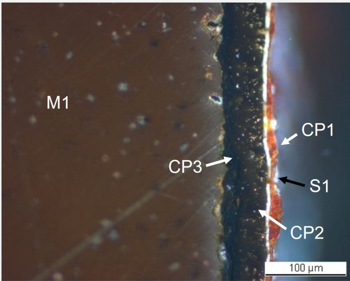
Fig. 12: Micrograph of the same area as Fig. 11 and corresponding to the stratigraphy of Fig. 14, polarized light. From left to right: metal (in brown) covered with a corrosion layer consisting of a black layer, an intermediate brown layer with bright spots, a crack (white line) and a red layer with white particles,
