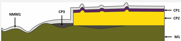
Fig. 5: Stratigraphic representation of the corrosion structure of the tang of a knife by macroscopic and binocular observation with reference to Fig. 4,
