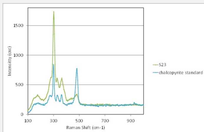
Fig. 18: Raman spectrum of the outermost layer (S23) of Fig. 14 compared to a chalcopryite standard spectrum. Settings: laser wavelength 532nm, acquisition time 50s, 4 accumulations, filter D2 (0.75-0.8mW), hole 1000, slit 100, grating 600. Method of analysis: Raman spectroscopy, Lab of Swiss National Museum, Affoltern a. Albis ZH,
