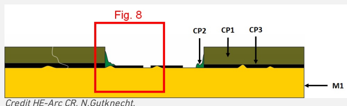
Fig. 7: Stratigraphic representation of the corrosion structure of the pin without head by macroscopic and binocular observation with indication of the corrosion structure used to build the MiCorr stratigraphy of Fig. 8 (red square),
