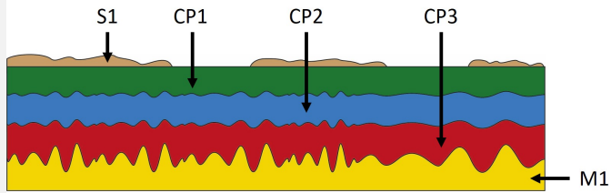
Fig. 3: Stratigraphic representation of the corrosion structure of the bracelet by macroscopic and binocular observation,
