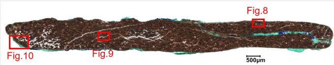
Fig. 6: Micrograph of the cross-section of the sample taken from the coin (Fig. 2) in dark field showing the location of Figs. 8 to 10,
