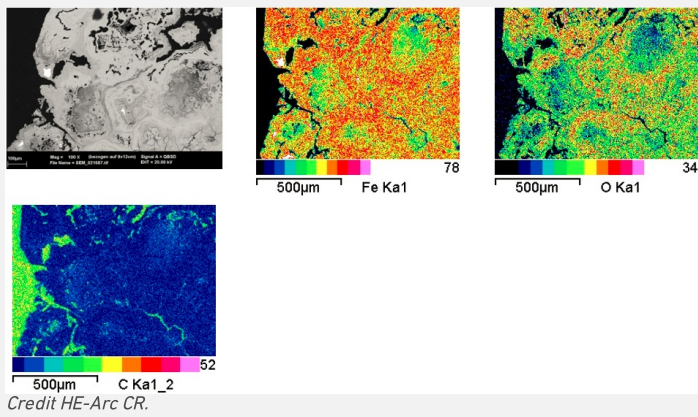
Fig. 13: SEM image, BSE-mode, and elemental chemical distribution of the selected area from Fig. 10 (rotated by 45°). Method of examination: SEM/EDS, Laboratory of Analytical Chemistry, Empa,
