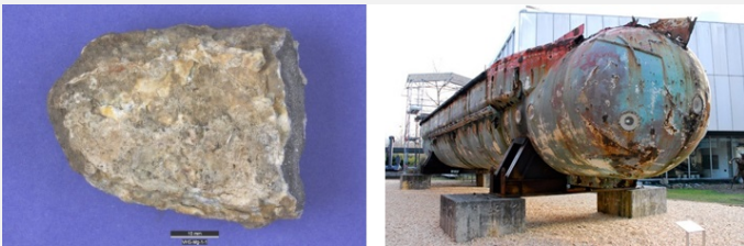
Fig. 1: Sacrificial anode (left) from submarine "Mesoscaph" (right) ( www.verkehrshaus.ch ),
