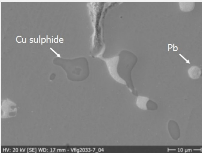
Fig. 6: SEM image (detail of Fig. 5), SE-mode, showing copper sulphide and lead inclusions,
