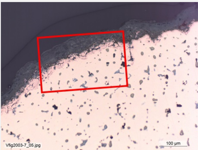
Fig. 5: Micrograph of the cross-section of sample from Fig. 2 of the headrest (or horse bit) (detail of Fig. 4), unetched, bright field. Light grey copper sulphide and tiny round Pb inclusions as well as "porosities" can be observed. Area of Fig. 9 is marked by a red rectangle,
