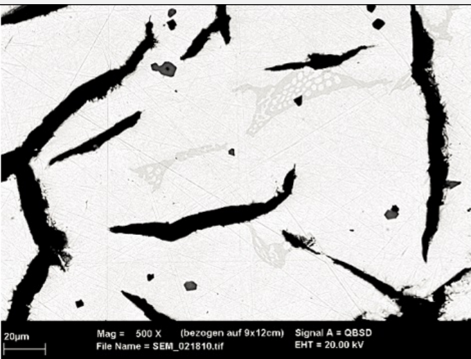
Fig. 5: SEM image from Fig. 3 (detail), BSE-mode, unetched. We observe the graphite flakes in black, the manganese sulphide inclusions in grey and the eutectic mixture in light-grey,
