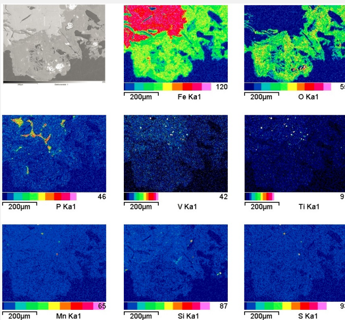
Fig. 10: SEM image, SE-mode, and elemental chemical distribution of the selected area from Fig. 3 (detail). Method of examination: SEM/EDS, Laboratory of Analytical Chemistry, Empa,
