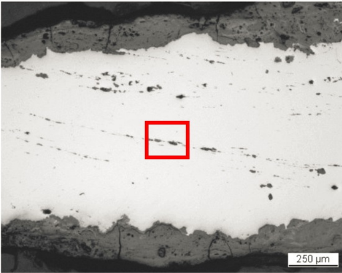
Fig. 4: Micrograph of the metal sample from Fig. 3 (detail), unetched, bright field. In white the metal, in light-grey the slag inclusions and the corrosion layer. The micrograph of Fig. 5 is marked by a rectangle,
