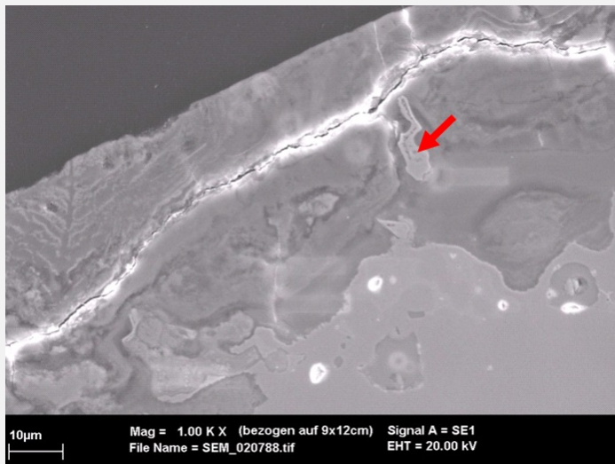
Fig. 6: SEM image of the metal sample (detail of Fig. 4, reversed picture), SE-mode. From bottom right to top left: the metal, the inner and outer corrosion layers separated by a large fissure. The red arrow indicates a remnant of the Sn-rich alpha-delta eutectoid.
