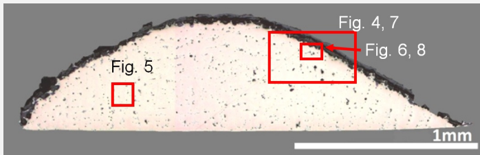
Fig. 3: Micrograph of the cross-section of the sample taken from the bracelet with uniform inclined rib showing the location of Figs. 4 to 8,
