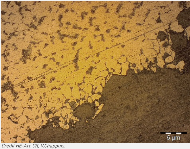
Fig. 8: Micrograph of the selected area of Fig. 7, Nital etched with no clear grain structure, bright field, Intergranular corrosion and grey phase (perlite?) are observed,
