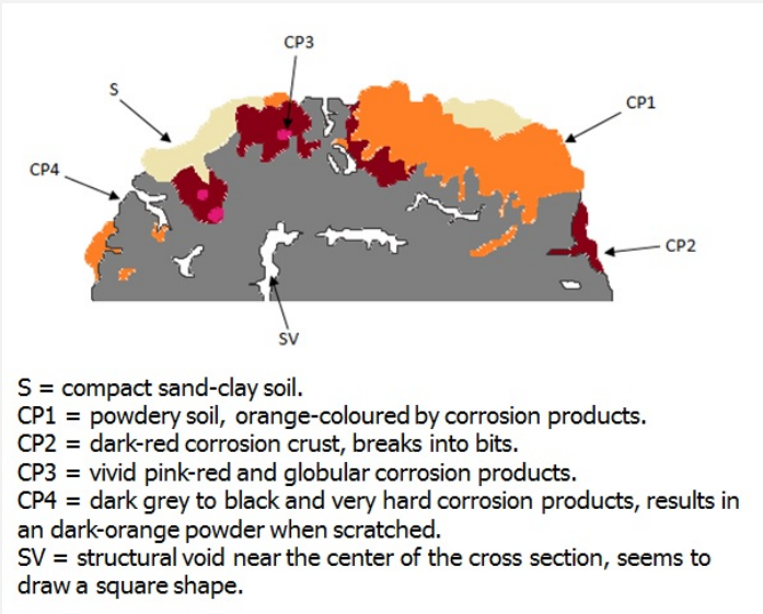
Fig. 3: Preliminary stratigraphy of the corrosion layers based on the observation of a broken nail,
