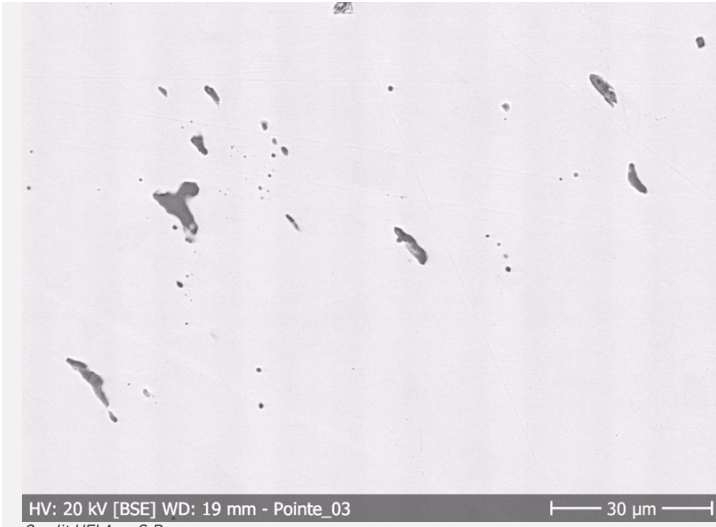
Fig. 6: SEM, BSE-mode picture of inclusions in remaining metal (detail of Fig. 5),
