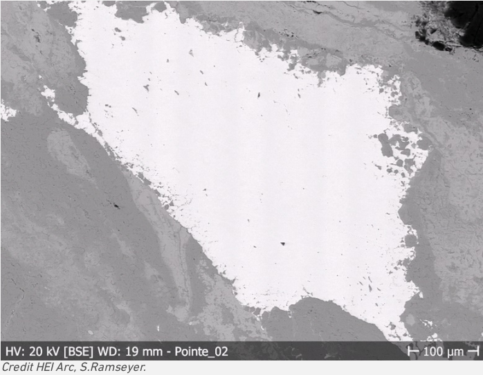
Fig. 5: SEM, BSE-mode picture of remaining metal from cross-section of Fig. 4,
