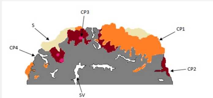
Fig. 3: Preliminary stratigraphy of the corrosion layers based on the observation of a broken nail,
