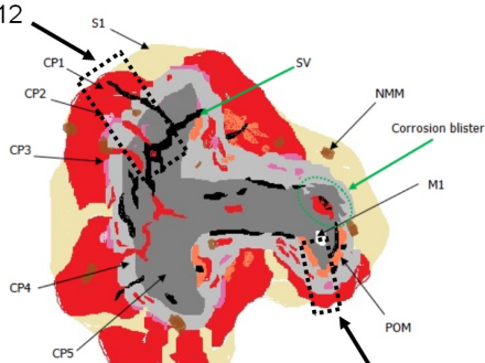
Stratigraphy, Fig. 13
