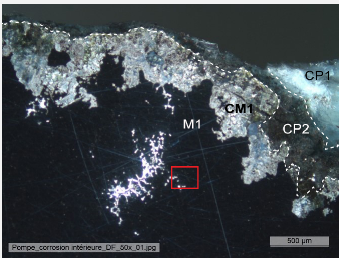
Fig. 8: Micrograph of the selected area (in red) of the sample shown on Fig. 7, unetched, dark field with location of Fig. 10,
