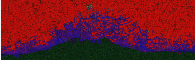
Fig. 14: SEM cartography of a pit of corrosion developing on the pipe. 20kV. Red = Al, Green = Cl, Blue = O,
