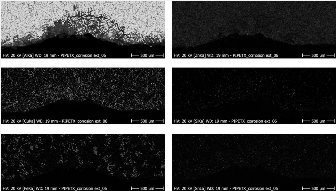
Fig. 11: SEM image and EDS elemental chemical distribution of main and interdendritic phases of the pipe. 20kV,
