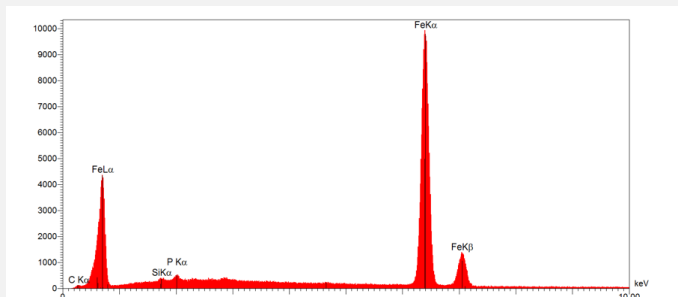
Fig. 5: EDS-spectrum showing the chemical composition of the metal (M1). The surface area analyzed was approx. 2*2 mm. Method of analysis: SEM-EDS. Lab. of Electronic Microscopy and Microanalysis, Néode, HEI Arc,
