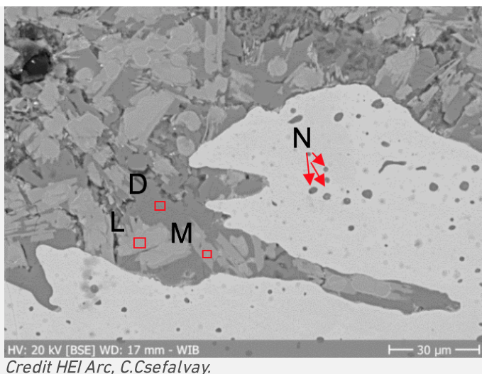
Fig. 7: SEM-image (BSE-mode) of the selected area from Fig. 6 (detail). The different phases in the slag inclusions are clearly visible: L = light grey phase, M = medium grey phase, D = dark grey phase/matrix, N = nodules,
