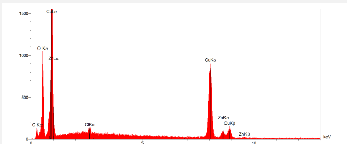
Fig. 9: EDS analysis of the red corrosion product. Method of analysis: SEM-EDS, Lab of Electronic Microscopy and Microanalysis, Néode, HEI Arc,
