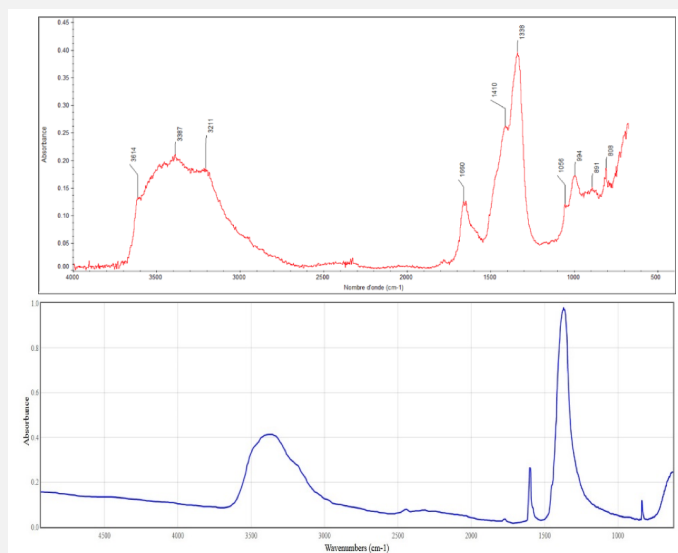
Fig. 10: FTIR spectrum (ATR mode) of the white corrosion product product (top), and of synthesized copper nitrate ( \text{Cu}(\text{NO}_3)_2 \cdot 3\text{H}_2\text{O} ) (bottom),
