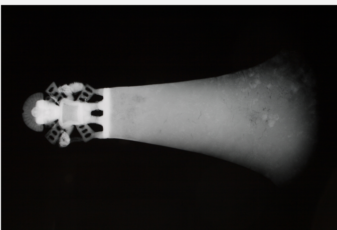
Fig. 12: X-ray radiography of the sacrificial knife showing how incrustations are put in place, the various thickness of the blade and its porosity (black holes on the right) as well as corroded areas (close to the cutting edge),
