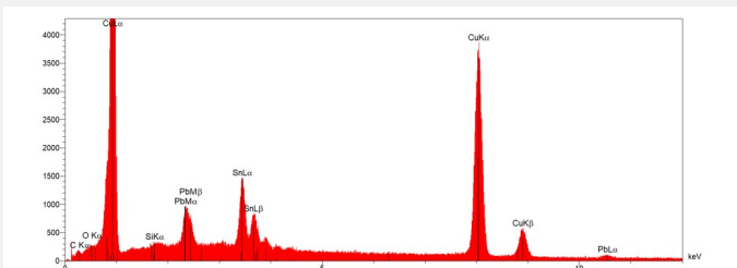
Fig. 12 : EDS spectrum of the alloy of the bracelet,
