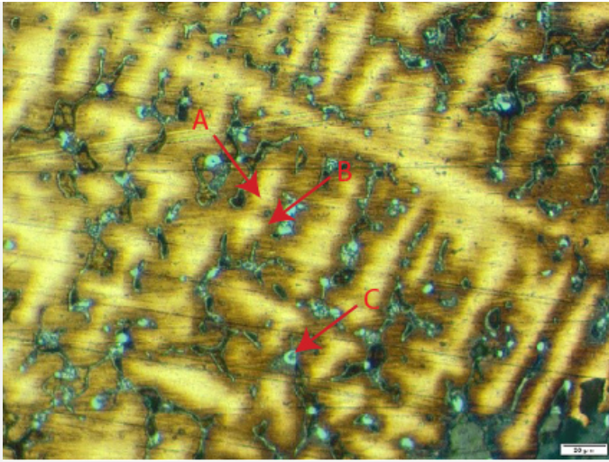
Fig. 14: Micrograph of a selected area of Fig. 13, etched, bright field, showing the dendritic (A), interdendritic (B) phases and lead nodules (C),
