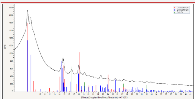
Fig. 21: XRD spectrum of the sample of the dark green corrosion product showing the presence of atacamite and paratacamite ( \text{Cu}_2\text{Cl}(\text{OH})_3 ) as major compound and cuprite ( \text{Cu}_2\text{O} ) as minor compound,
