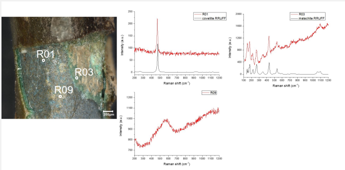
Fig. 6: Raman points of analysis on the surface of the object and Raman spectra obtained for R01(together with the covellite reference spectrum RRUFFID=R060306), R03 (together with the malachite reference spectrum RRUFFID=R050508) and R09,
