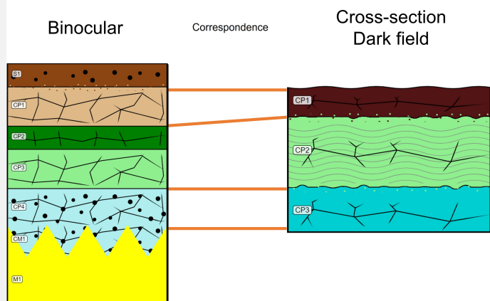
Fig. 8: Stratigraphic representation side by side of binocular view and cross-section (dark field),
