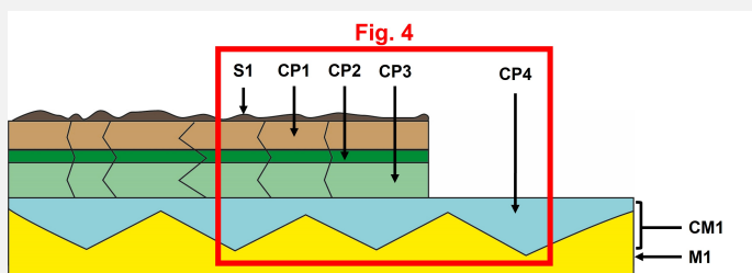
Fig. 3: Stratigraphic representation of the corrosion structure of the pin by macroscopic and binocular observation with location of Fig. 4,
