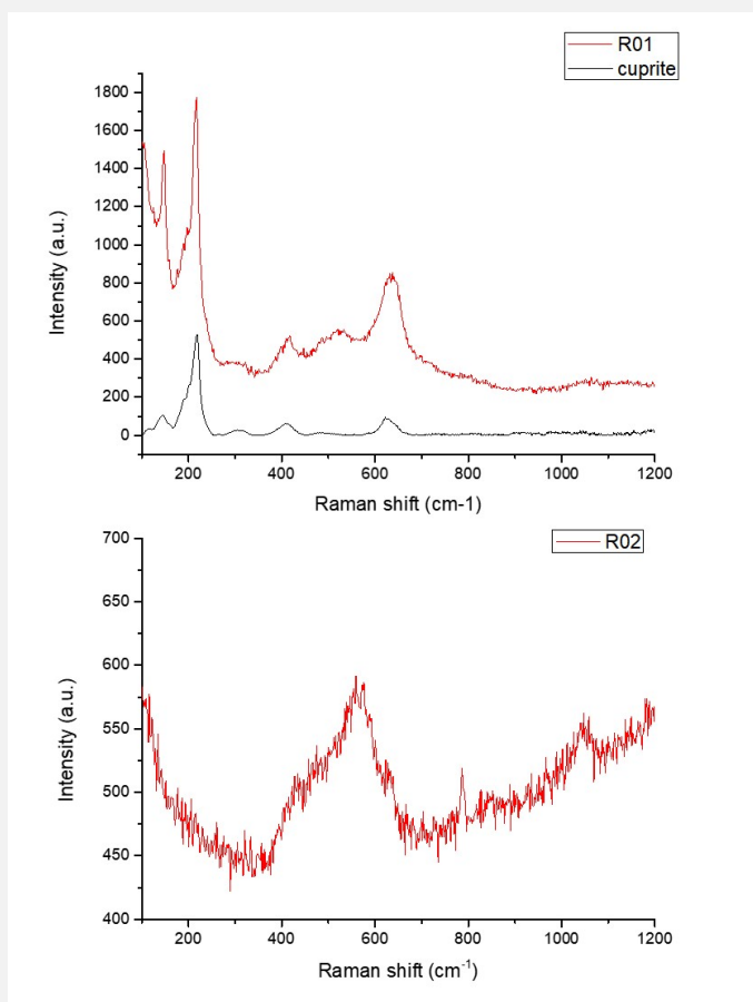
Fig. 11: Raman spectra of points R01 (together with the RRUFF reference RRUFFID=R140763 for cuprite) and R02 shown in Fig. 10,
