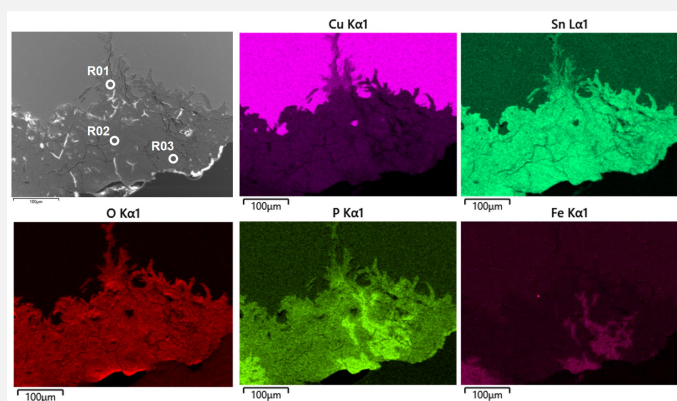
Fig. 11: SEM image, BSE-mode, and elemental chemical distribution of Fig.10. The selected points for Raman analysis shown in Fig. 12 are indicated,
