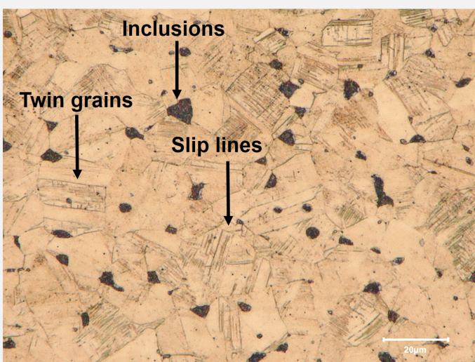
Fig. 7: Micrograph of the metal sample from Fig. 5 (detail), etched, bright field. Elongated grains with slip lines are observed, as well as grey lead inclusions,
