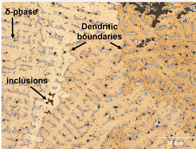
Fig. 7: Micrograph of the metal sample from Fig. 5 (detail), etched, bright field, dendritic structure. Presence of grey Sn-rich \alpha+\delta phase and black Pb inclusions,
