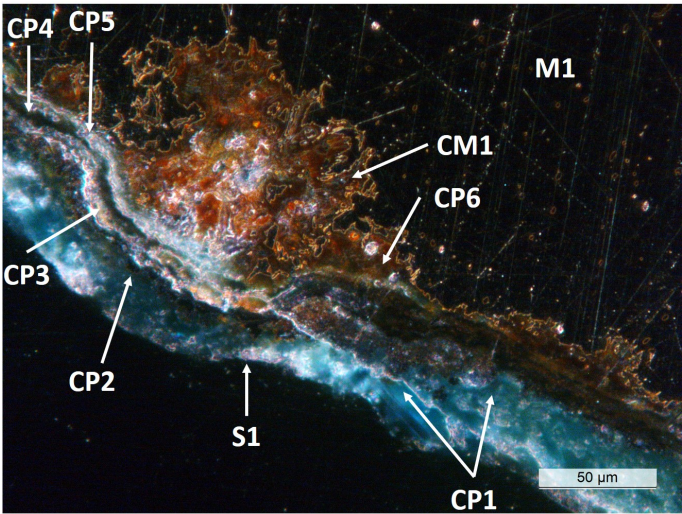
Fig. 18: Micrograph of the metal sample similar to Fig.17 (detail), unetched, dark field, and corresponding to the stratigraphy of Fig. 21,
