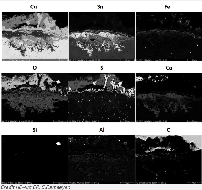
Fig. 15: Elemental chemical distribution of Fig. 14 (reversed). Method of examination: SEM/EDS, Microcity,
