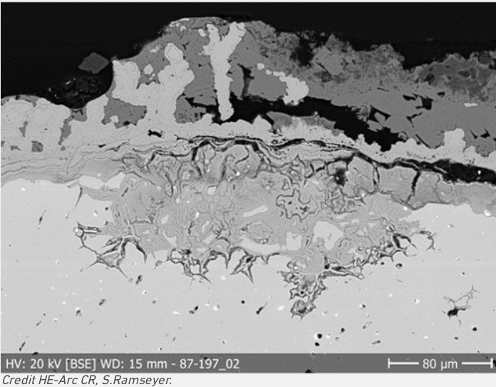
Fig. 14: SEM image, BSE-mode (detail of Fig. 12),
