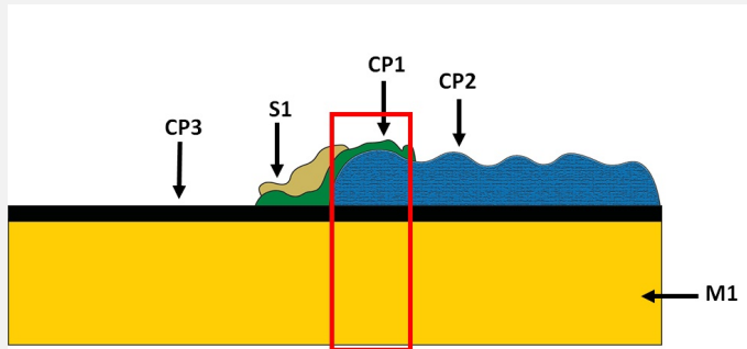
Fig. 4: Stratigraphic representation of the corrosion structure of the coin by macroscopic and binocular observation with indication of the corrosion structure used to build the MiCorr stratigraphy of Fig. 5 (red square),
