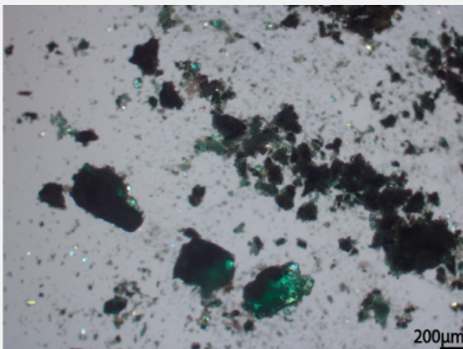
Fig. 14: Dark green corrosion product identified as paratacamite, atacamite \text{Cu}_2\text{Cl}(\text{OH})_3 by XRD. Microscopic examination under polarized light,
