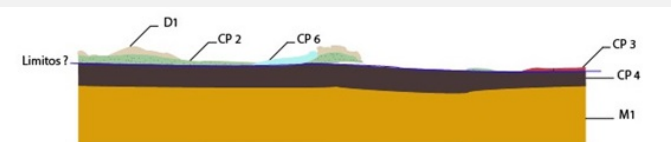
Fig. 8: Preliminary stratigraphy 3, corresponding to the area of the back face of the aegis with a well-preserved limit of original surface. S = soil, D = deposit, M = metal, CP = corrosion products,
