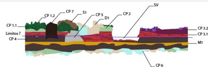
Fig. 7: Preliminary stratigraphy 2, corresponding to the back face of the aegis and interior (below part). S = soil, D = deposit, M = metal, CP = corrosion products, SV = structural void,
