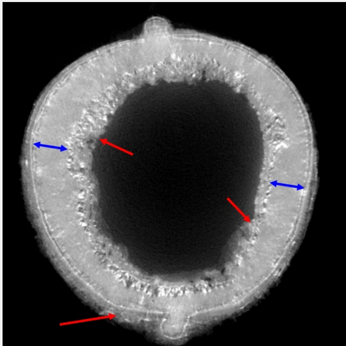
Fig. 11: X-ray tomography by cross section of the crown showing a dense and non-porous metal core (blue arrows). The corrosion products however are porous (red arrows). The external limitos is visible as a fine line preserved under corrosion layers,
