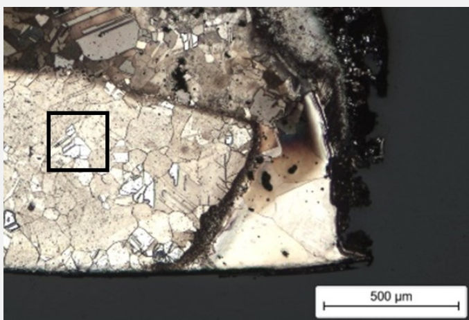
Fig.14 : Micrograph of the sample after etching. Twin lines are clearly visible in the black square,
