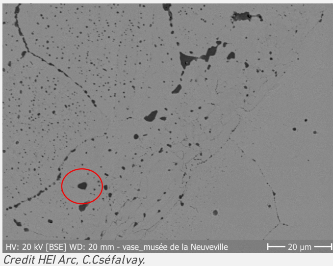
Fig. 11: SEM picture (BSE mode) of the metal sample from Fig. 9 (detail), with copper inclusion,
