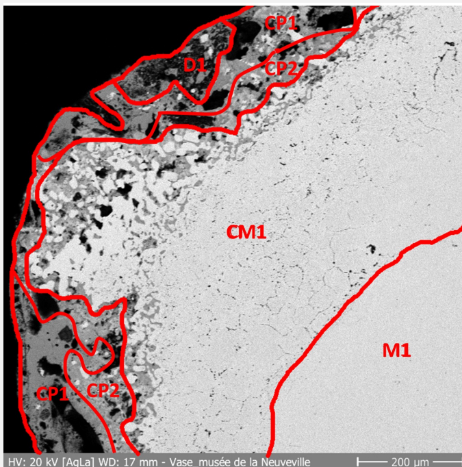
Fig. 16: Elemental distribution of Ag within the corrosion structure from Fig. 15 (detail) with the subdivision of the different strata,
