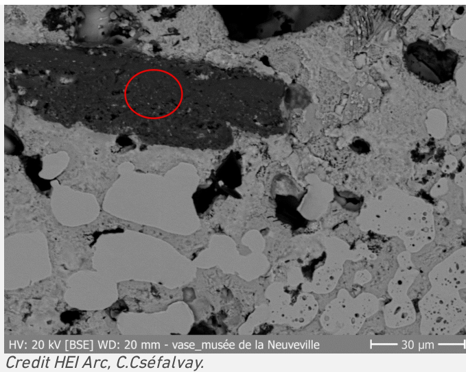
Fig. 12: SEM picture (BSE mode) of the metal sample from Fig. 9 (detail), with iron inclusion,
