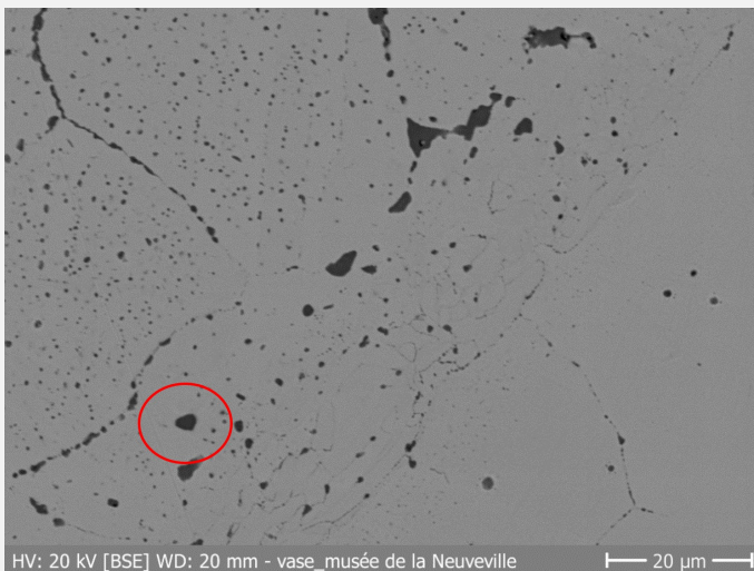
Fig. 11: SEM picture (BSE mode) of the metal sample from Fig. 9 (detail), with copper inclusion,
