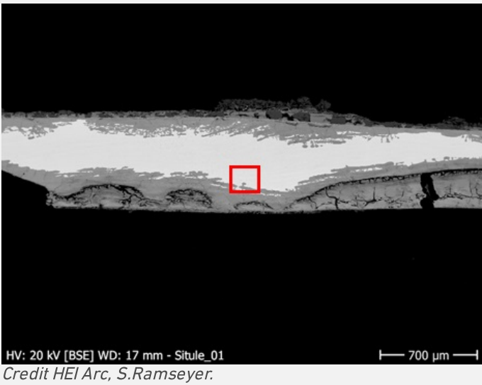
Fig. 5: SEM image, BSE-mode, of the metal sample from Fig. 4. Area of Fig. 6 is marked by a red square,
