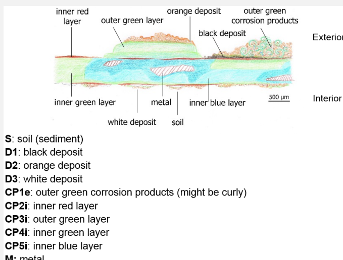
Fig. 3: Stratigraphic representation of the situla by macroscopic observation,
