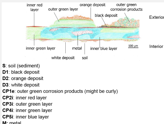
Fig. 3: Stratigraphic representation of the situla by macroscopic observation,
