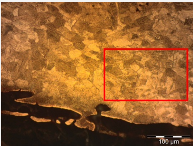
Fig. 6: Micrograph of the metal structure from Fig. 5 (detail), etched, bright field, 50x. The alpha phase of the alloy shows polygonal grains. Area of Fig. 7 is marked by a red rectangle,
