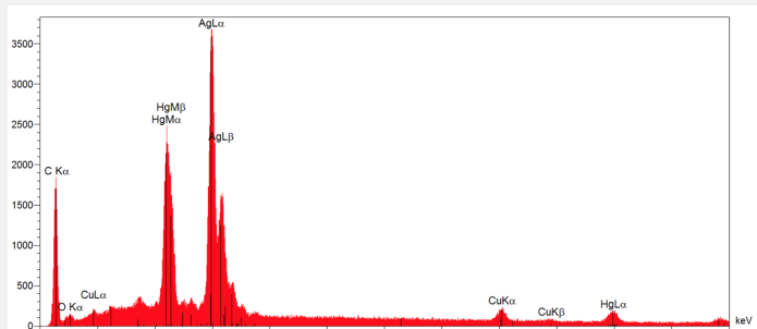
Figs. 10: EDS analysis of the layer that appears light grey under polarized light, situated below the red layer (Fig. 4). Method of analysis: SEM-EDS, Lab of Electronic Microscopy and Microanalysis, IMA (Néode), HEI Arc,
