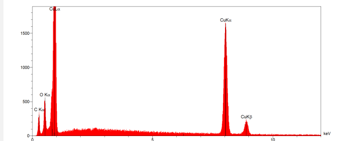
Fig. 9: EDS analysis of the red corrosion layer (Fig. 4). Method of analysis: SEM-EDS, Lab of Electronic Microscopy and Microanalysis, IMA (Néode), HEI Arc,
