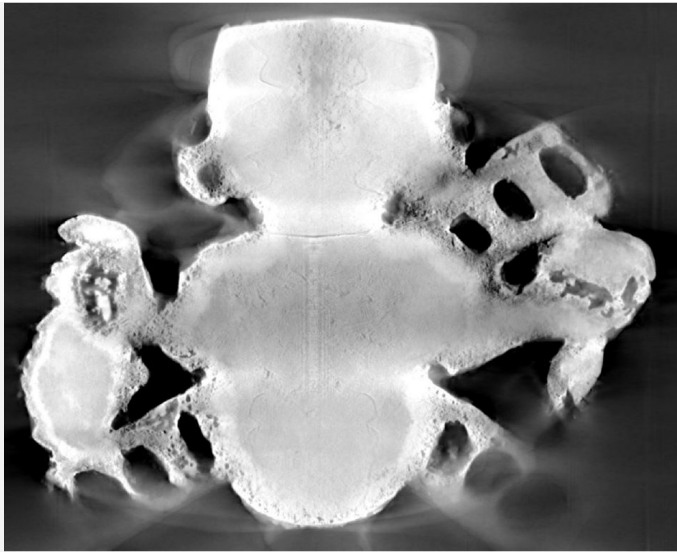
Fig. 13: X-ray tomography of the handle decorated with a character of the sacrificial knife indicating the porosity of the metal,
