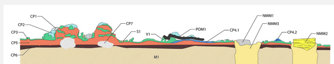
Fig. 14: Improved representation of the stratigraphy of corrosion layers of the sacrificial knife from visual observations and analyses,
