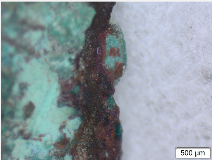
Fig. 8: Broken edge of the blade (see Fig. 4), showing the different corrosion layers in cross-section,
