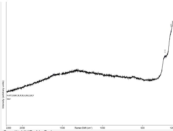
Fig. 18: Raman spectrum of the mineralised metal sample (Fig. 8) possibly silver chloride,
