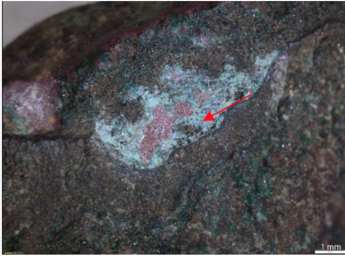
Fig. 15: Observation of the light green corrosion product,
