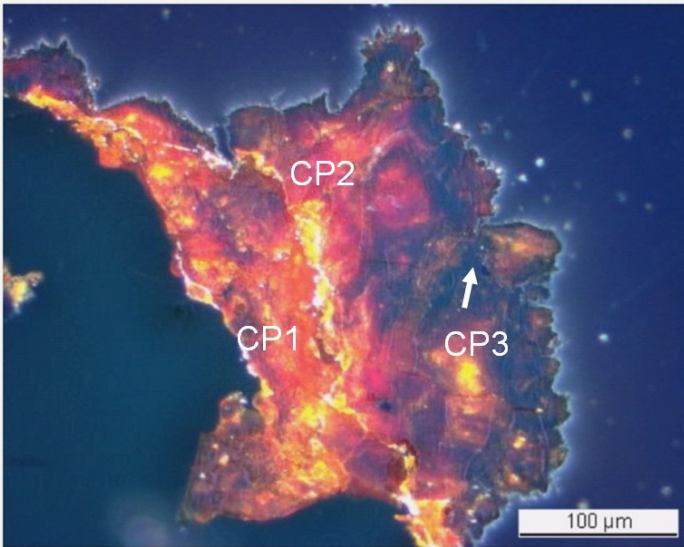
Fig. 9: Micrograph showing the metal - corrosion crust (same as Fig. 8) and corresponding to the stratigraphy of Fig. 11, unetched, polarised light. The corrosion products are dark-brown at the metal - corrosion crust interface and red-orange on the outside,
