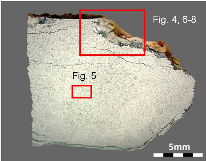
Fig. 3: Micrograph of the cross-section of the fragment sampled from the sacrificial anode showing the location of Figs. 4 to 8,
