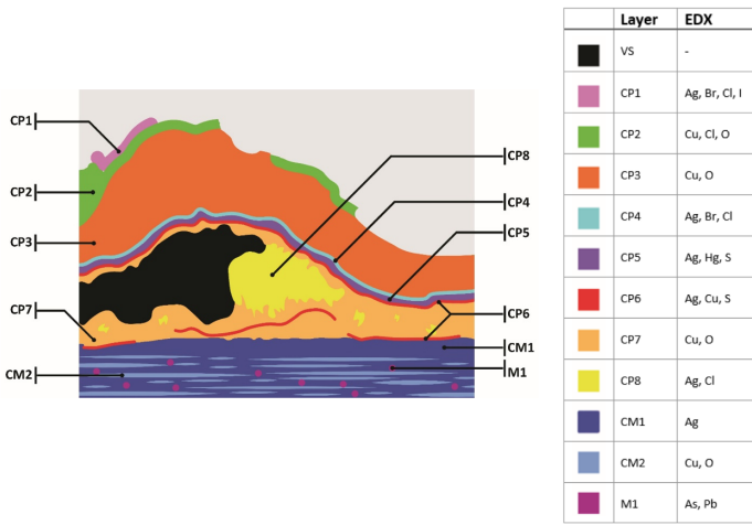
Fig. 17: Improved stratigraphic representation of the funeral mask (Fig. 3) based on the results from the SEM-EDS analyses,
