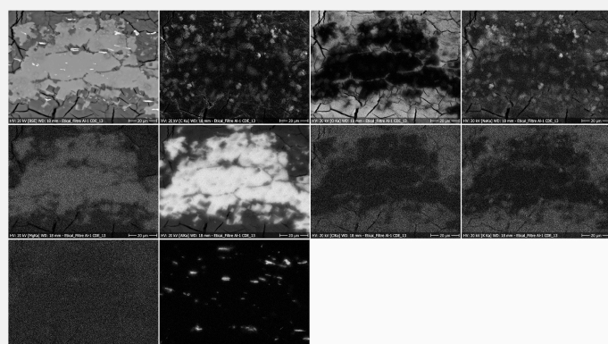
Fig. 11: SEM image, BSE-mode, and elemental chemical distribution of the selected area of Fig. 8 reexamined after 4 months: new forms of alteration with a local enrichment of Na, C and O are observed,
