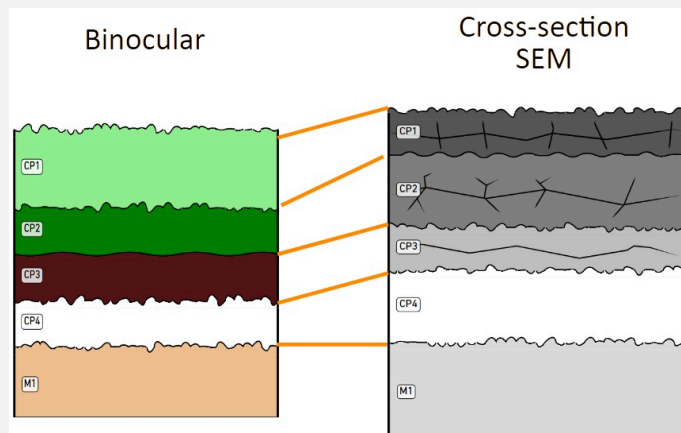
Fig. 16: Stratigraphic representation side by side of binocular view and cross-section (SEM),
