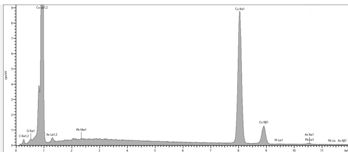
Fig. 7: EDS analysis of the metal. Mostly Cu and As with traces of Pb are found,
