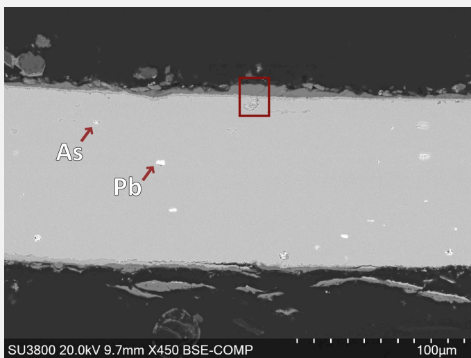
Fig. 8: SEM image, BSE-mode, of the metal sample from Fig. 2 with location of Fig. 9 (red square). Light-grey (As) and white (Pb) inclusions are distributed evenly,
