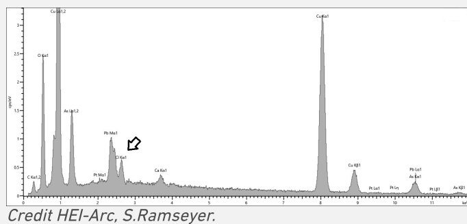
Fig. 12: EDS analysis corresponding to spectrum 42 - CP6 (Fig. 9),
