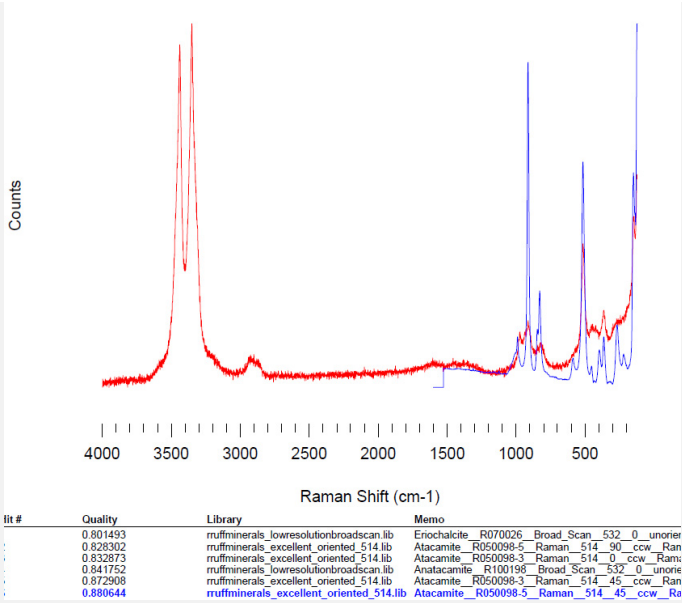
Fig. 13: Raman spectrum of CP1 and comparison with Ruffminerals database,
