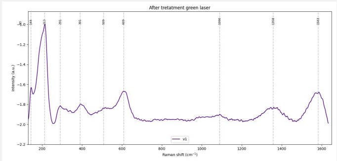
Fig. 14: Raman spectrum of CP3 and CP4,
