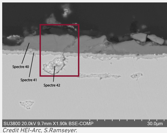
Fig. 9: SEM image of Chlorid corrosion roots, BSE-mode (detail of Fig. 8), spectrum 40 is detailed in Fig. 10, spectrum 41 is detailed in Fig. 11 and spectrum 42 is detailed in Fig. 12. Powdery compounds on top might be atacamite but were not analysed by EDS,
