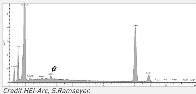
Fig. 11: EDS analysis corresponding to spectrum 41 - CP5 (Fig. 9),
