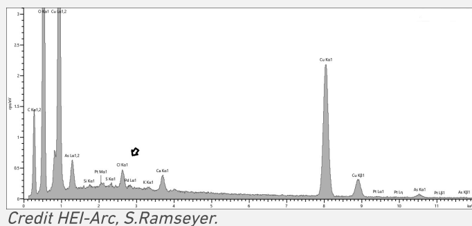
Fig. 10: EDS analysis corresponding to spectrum 40 - CP2 (Fig. 9),
