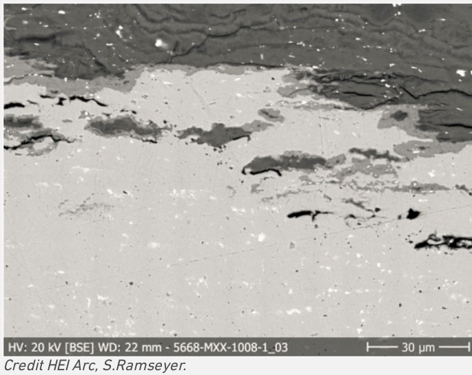
Fig. 6: SEM image of the cross-section, from Fig. 5 (detail), BSD-mode,
