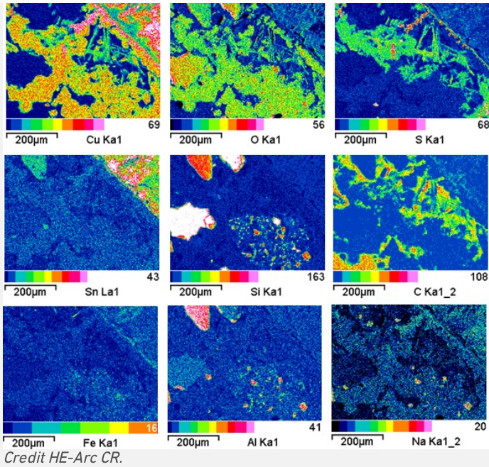
Fig. 10: EDX elemental chemical distribution of the SEM image of Fig. 8. Method of examination: SEM/EDX, Laboratory of Analytical Chemistry, Empa,
