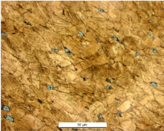
Fig. 5: Micrograph of the metal sample from Fig. 3 (detail), etched, bright field. We observe elongated grains with slip lines as well as grey copper sulphide inclusions,
